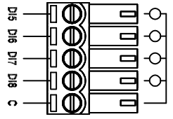
TB2
