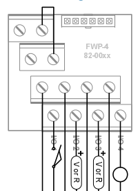
82-00xx or 82-01xx Field Wiring Panel
