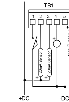
FIGURE A 20mA Sensors External Loop Supply
