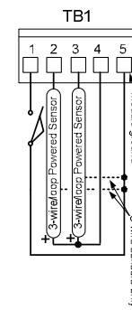
FIGURE B Sensor Power from Discrete Output
