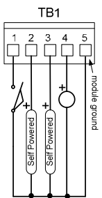
FIGURE C Self-powered 20mA Sensors
